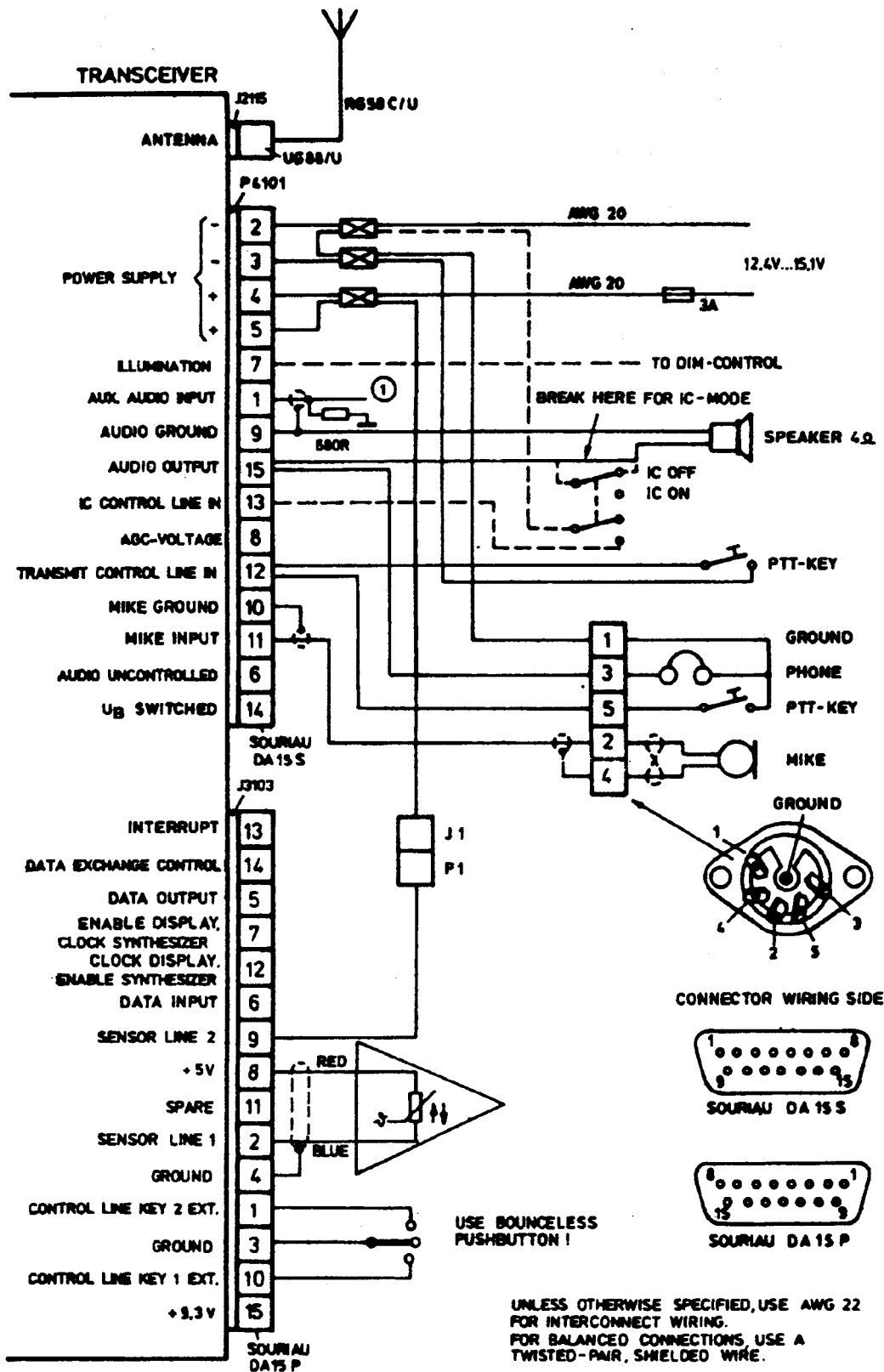
Fig. 2-5 Aircraft wiring
