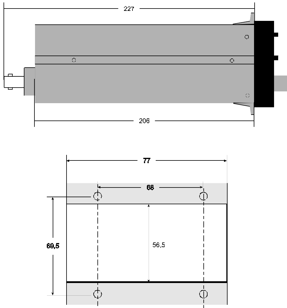
Figure 2.3 Outline and mounting Drawing
