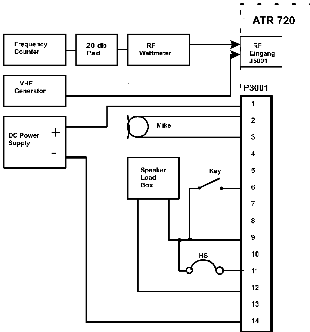
2-1 BENCH TEST SET-UP
