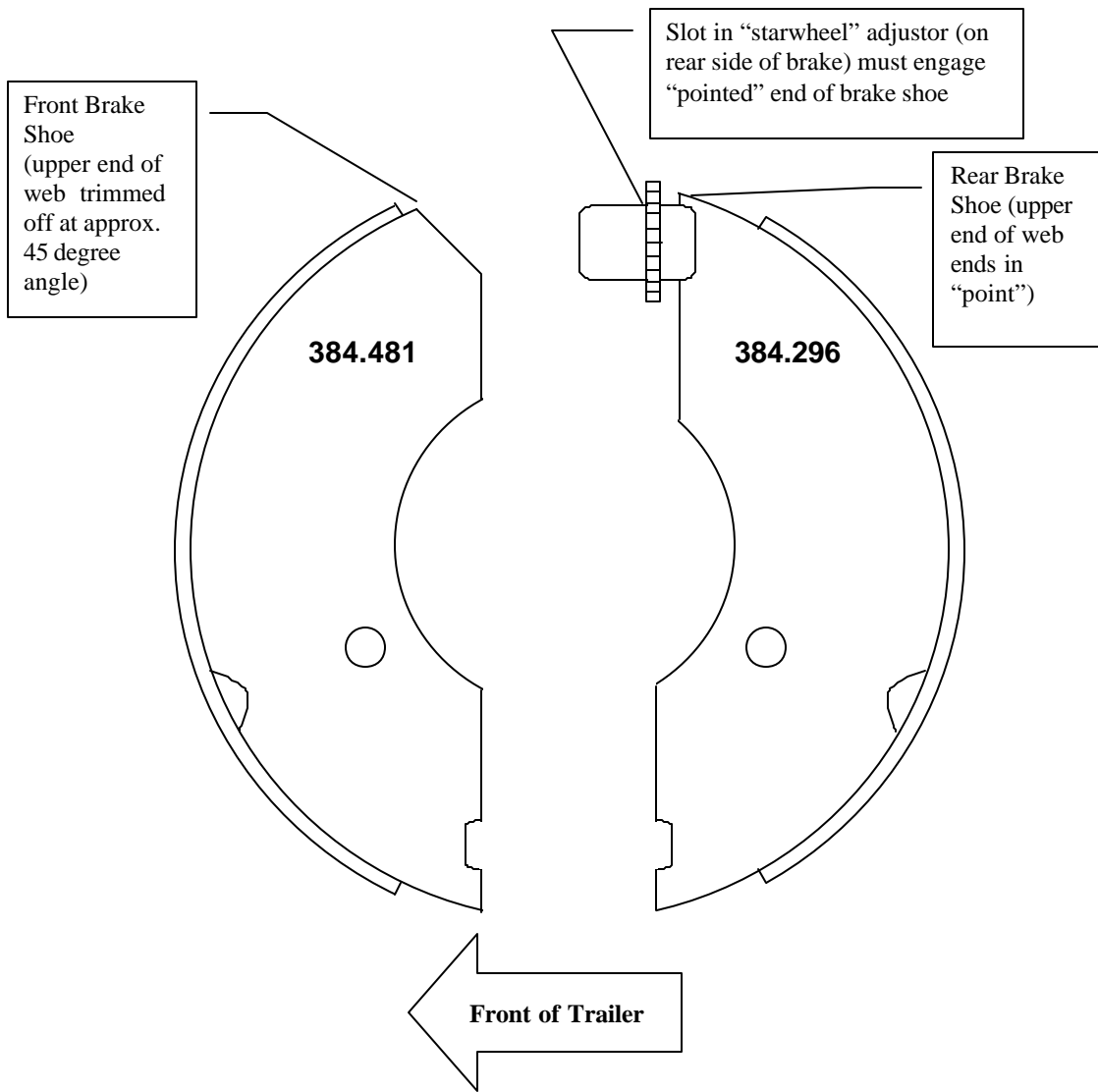
Brake Shoe Diagram for Type 1637 AL-KO Brake on Cobra Trailer (not to scale; consult factory maintenance manual for correct instructions and specifications; failure to heed factory instructions may result in loss of braking power, loss of automatic reversing capability, and/or brakes not releasing)
