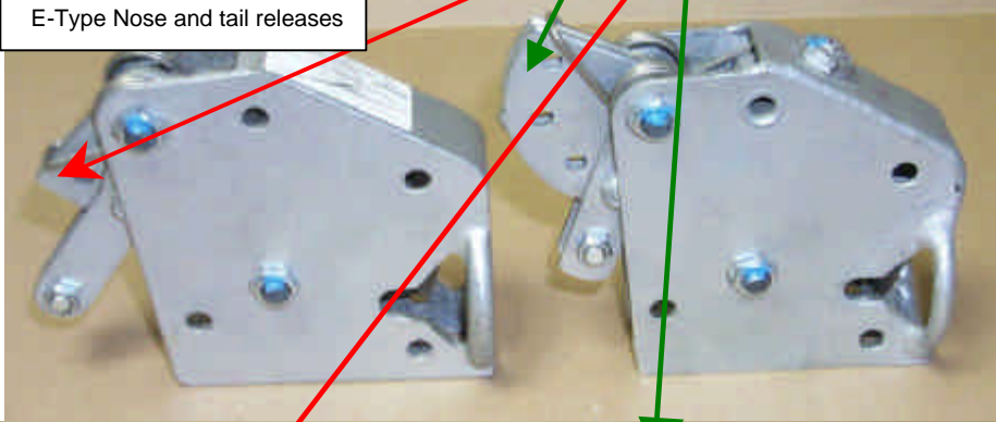
S-Type CG releases
