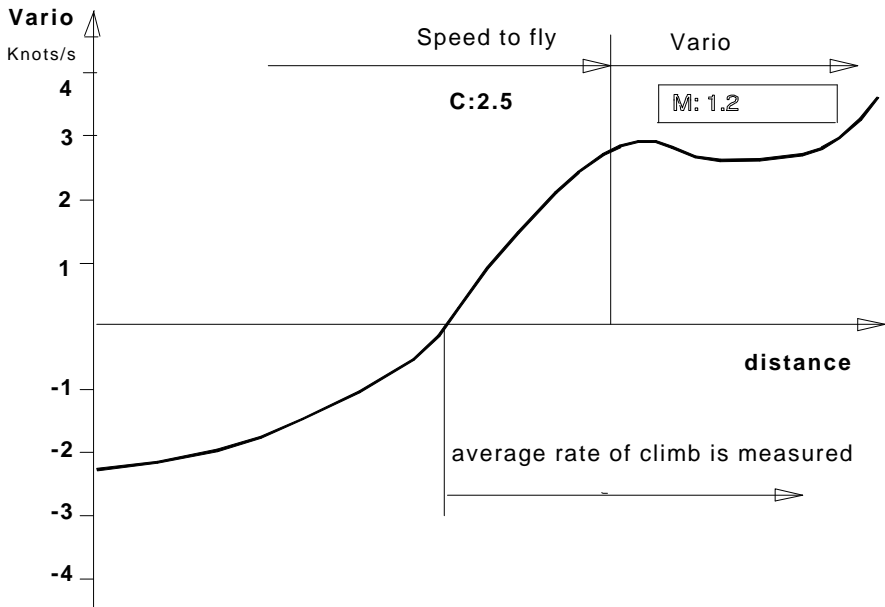
Fig. of 3.2-1: Average Rate of Climb (start of data capture)
