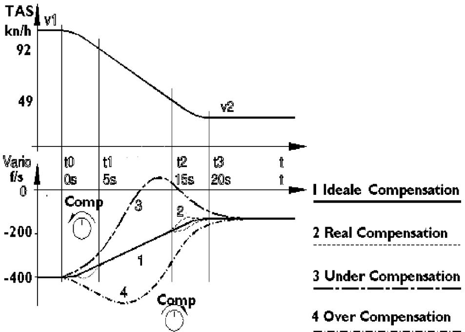
Fig. 7.2-1: Total-energy-Compensation
