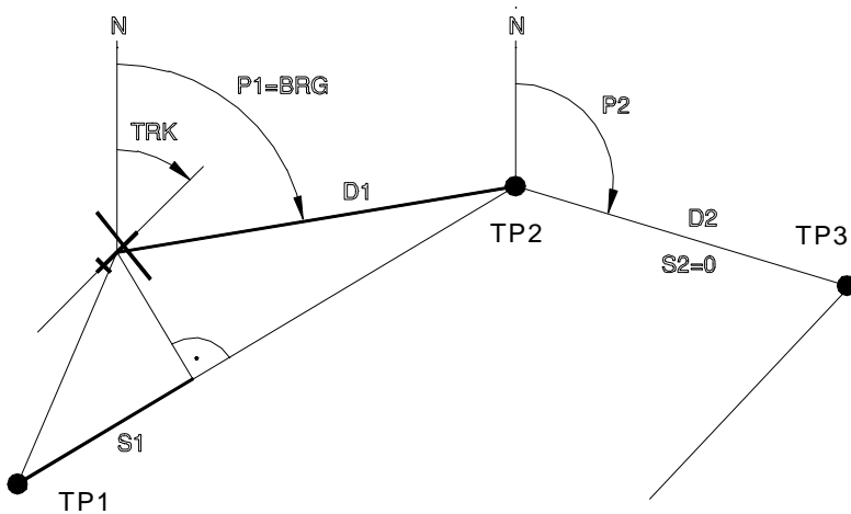
Fig. 4.3.1-1: Schematic depiction of the indicated sizes at active route of leg 1 (S1), distance D1, TRK = track (course over ground), P1 = BRG = bearing (bearing to the turn point of TP2), distance D2= distance from TP2 to the turn point TP3 (yet not active), bearing of P2 is the bearing between both these points.
