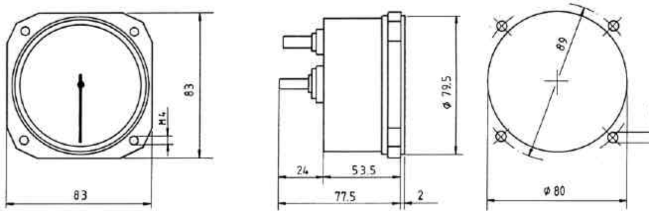
Airspeed indicators 7 FMS 2 und 7 FMS 5, pitot-tube airspeed indicator 7 FMS 4, UL-airspeed-indicator EBF
