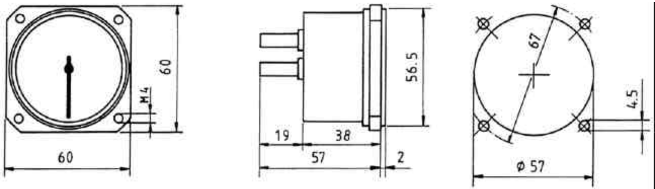
Airspeed indicators 7 FMS 2 und 7 FMS 5, pitot-tube airspeed indicator 7 FMS 4, UL-airspeed-indicator EBF
