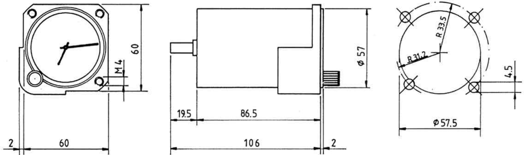
standard precision altimeter 4 FGH 40
