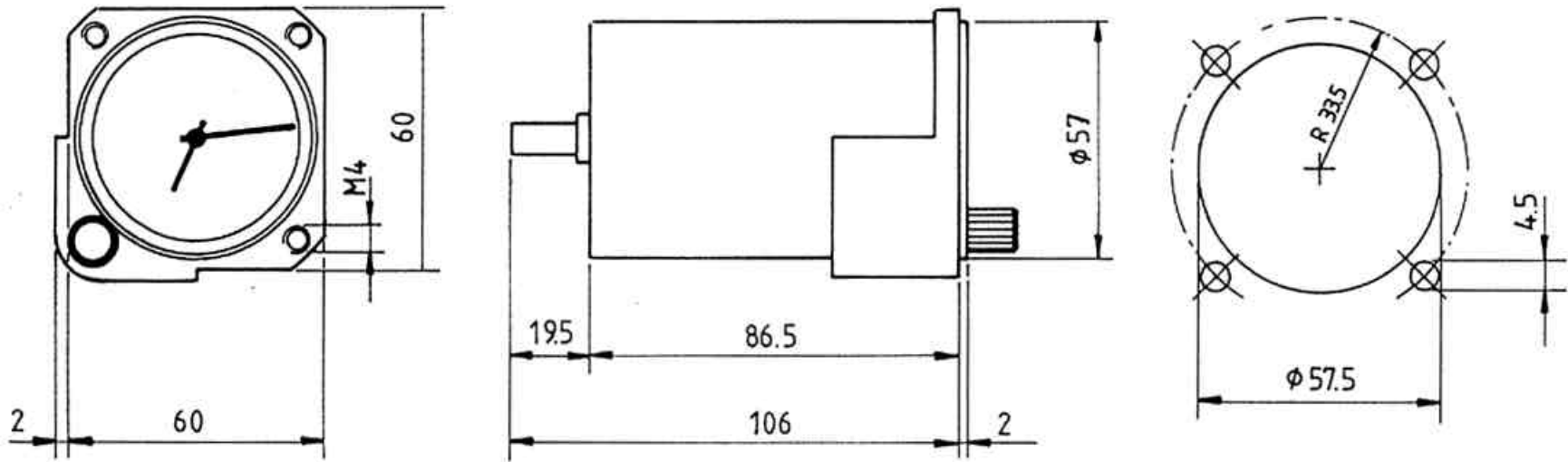
standard precision altimeter 4 FGH 40
