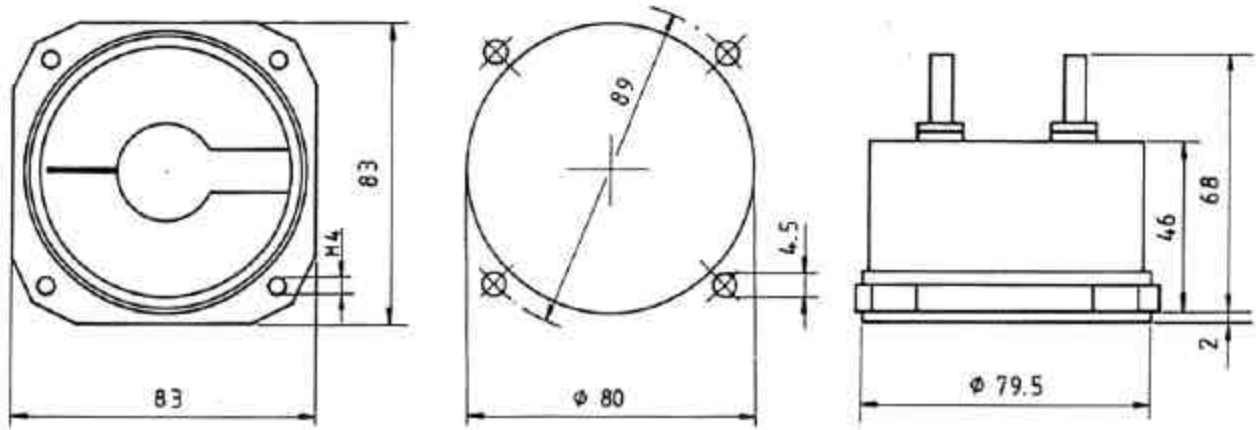
vane type variometers 5STVM5 and 5STVM10, UL-variometer EBV ±5M/S, UL-variometer EBV ±10M/S, UL-variometer EBV ±2000FT/MIN
